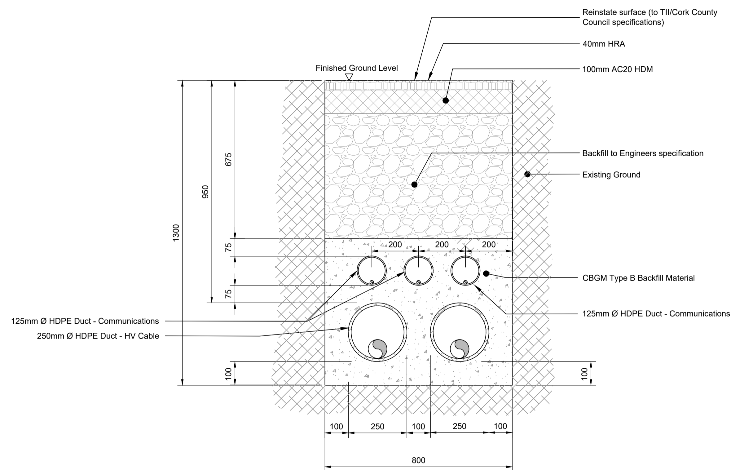
DC Cable - Typical Section 1:10
